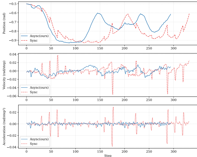
Fig. 9. Comparison of motion trajectories for Joint 4 of the UR robot between synchronous and asynchronous inference. Asynchronous inference results in smoother trajectories and reduced execution time.
